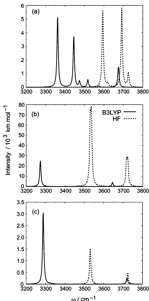
Figure 4. B3LYP and HF vibrational spectra in the O–H stretching region for (a) the AA isomer of (\text{H}_2\text{O})_4^- , (b) the cyclic isomer of (\text{H}_2\text{O})_4^- , and (c) the cyclic isomer of (\text{H}_2\text{O})_4 . Each panel uses a different intensity scale.
