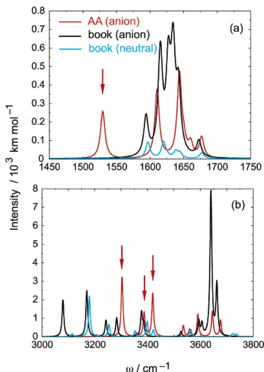
Figure 5. B3LYP vibrational spectra in (a) the H–O–H bending region and (b) the O–H stretching region, for isomers of (\text{H}_2\text{O})_6 and (\text{H}_2\text{O})_6^- . Arrows indicate normal modes with significant contributions from the AA water molecule.
